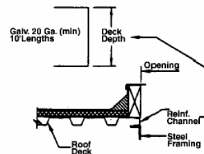
REINFORCING CHANNEL
