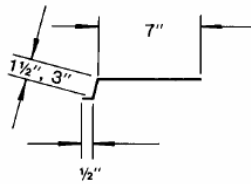
FILLER SHEET (20 GA.) 10'-0" LENGTHS GALVANIZED ONLY
