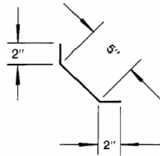
CANT STRIP (20 GA.) 10'-0" LENGTHS GALVANIZED ONLY
