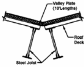
VALLEY DETAIL
