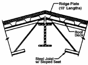
RIDGE DETAIL
